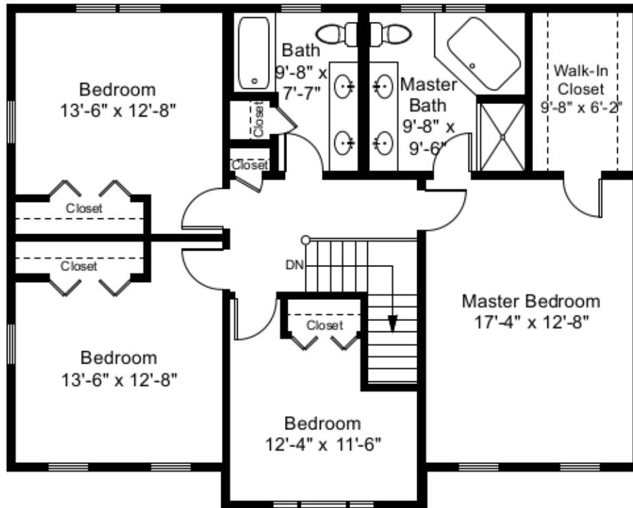
Second Floor Plan Ceiling Height = 8'-0"
