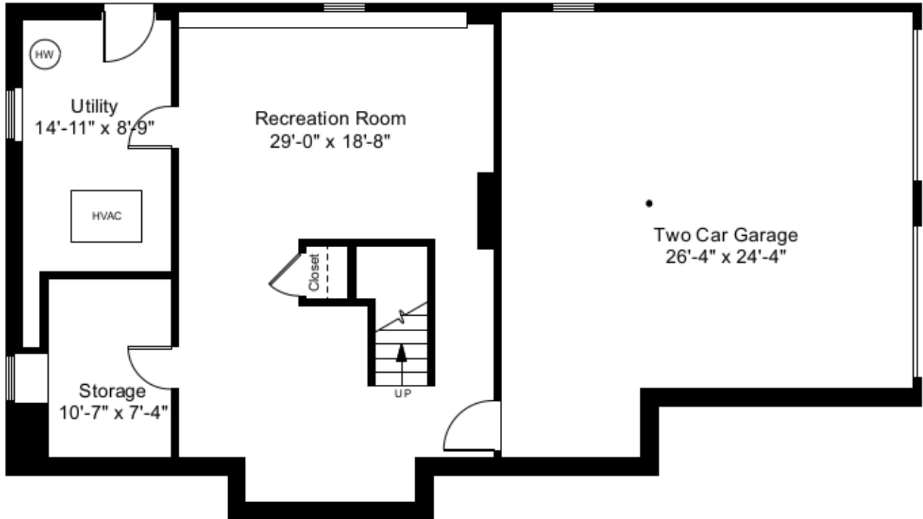
Lower Level Plan Ceiling Height = 6'-9"
