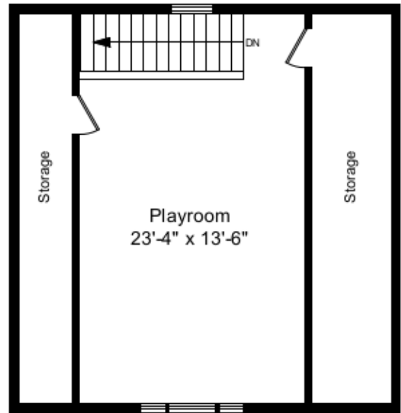
Garage - Second Floor Plan Ceiling Height = 8'-2"
